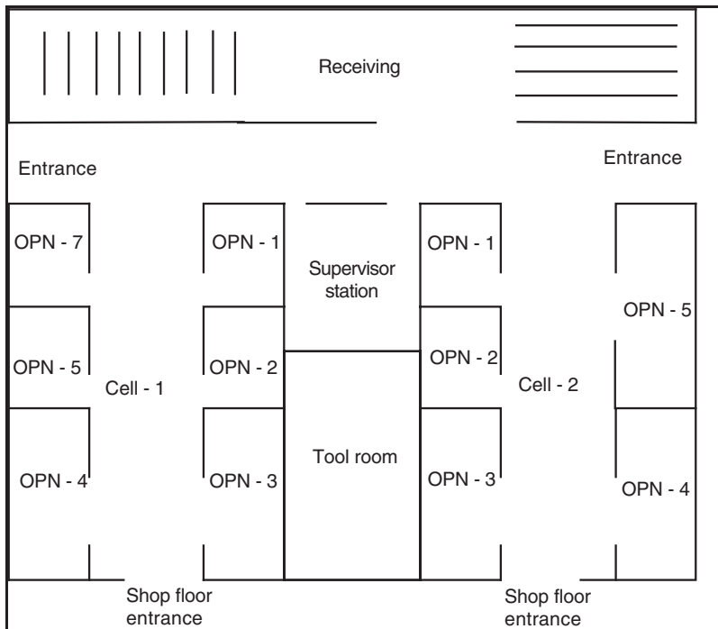
FIGURE 23.2 Facility layout for scoping network requirements.
