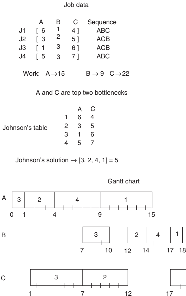
FIGURE 32.7 A heuristic approach to schedule a job shop. Compare with other guesses and pick lowest C_{\max} .
