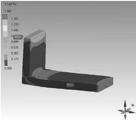
FIGURE 28.18 Equivalent stress and deformation obtained from VAA service.
