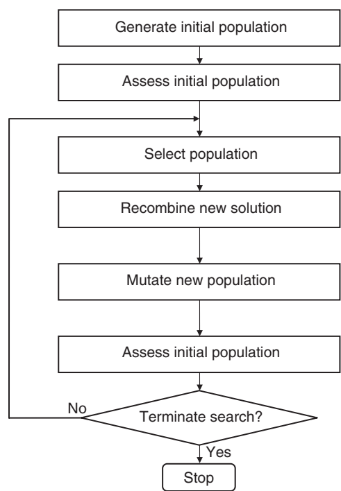
FIGURE 22.6 The basic structure of a genetic algorithm.
