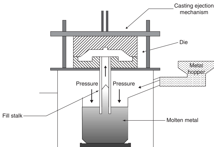
FIGURE 15.2 Die casting.
