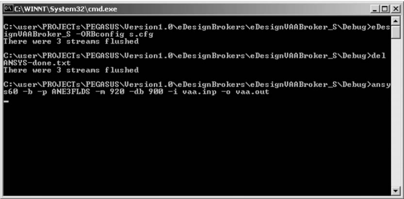
FIGURE 28.17 VAA service provider.
