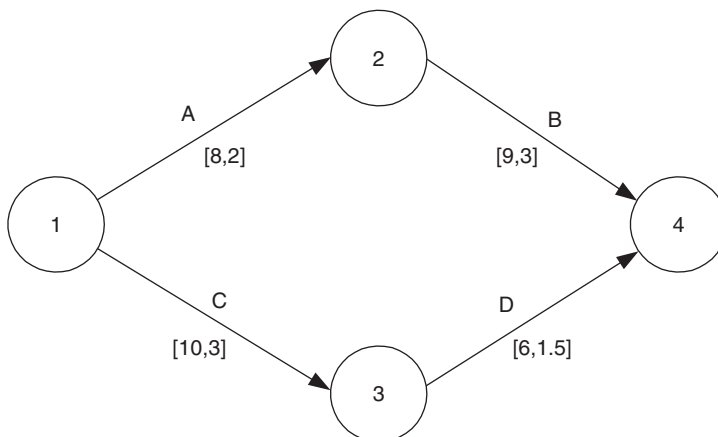
FIGURE 4.35 Stochastic network.
