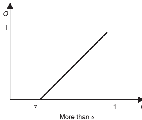
FIGURE 24.2 Satisfaction level of the “More than \alpha ” linguistic quantifier.
