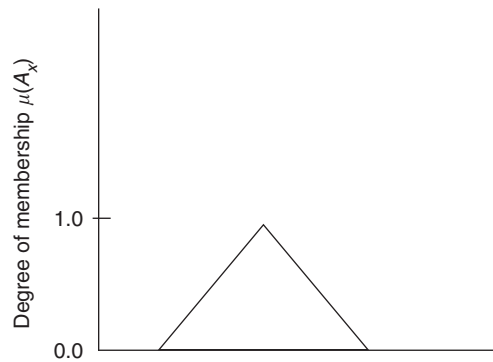
FIGURE 25.6 Triangular membership function.
