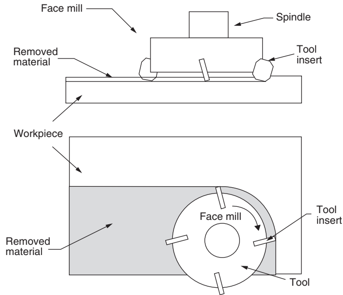
FIGURE 15.7 Face milling.
