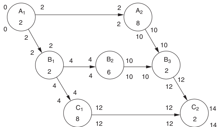
FIGURE 4.31 AON network of partitioned activities (from Badiru and Pulat, 1995).
