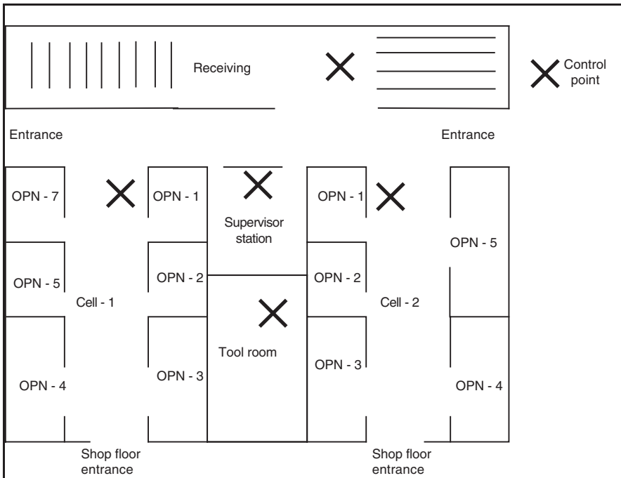
FIGURE 23.6 Control point diagram.
