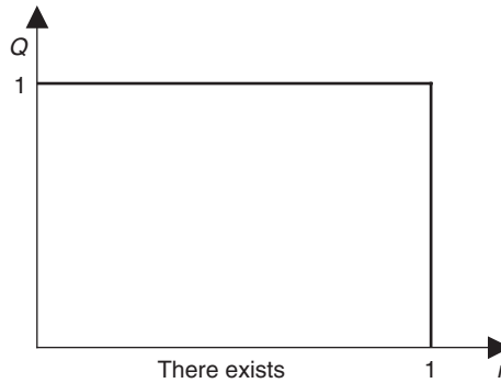
FIGURE 24.1 Satisfaction level of the “There exists” linguistic quantifier.
