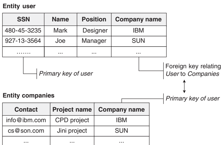
FIGURE 20.3 Relational tables.
